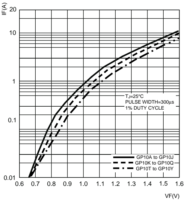
FIG.3 典型正向特性曲线 TYPICAL FORWARD CHARACTERISTICS
