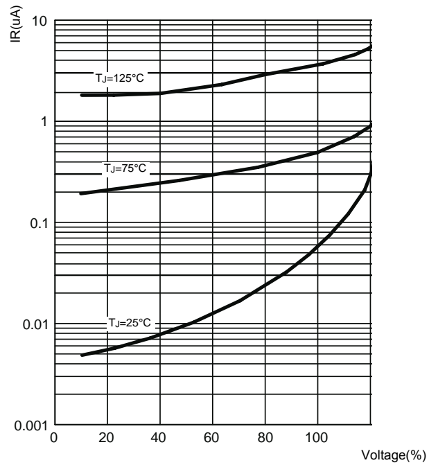
FIG.4 典型反向特性曲线 TYPICAL REVERSE CHARACTERISTICS
